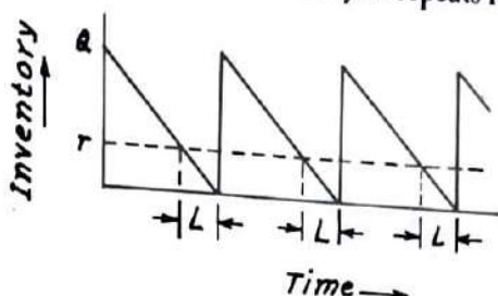
Fig. 24.3. Time pattern for inventory level for simple EOQ model.
