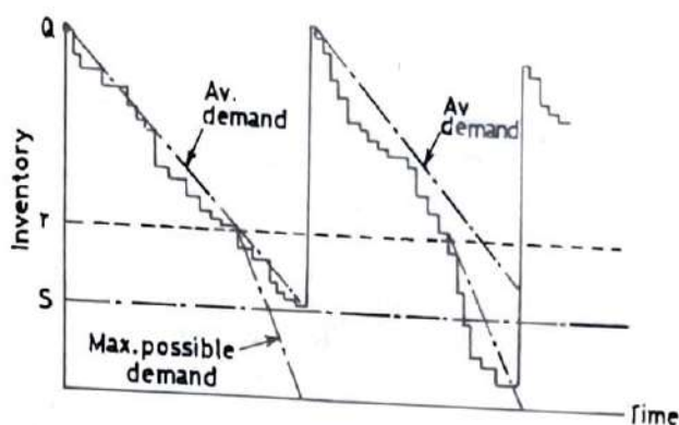
Fig 24.5. Inventory levels under conditions of fluctuating demand.
